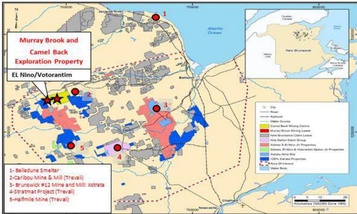
Murray Brook Project and Camel Back property location map, Bathurst Mining Camp, New Brunswick.
