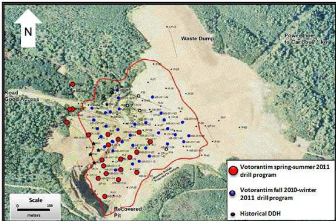
Figure 2- Plan view showing outline of the Murray Brook polymetallic massive sulphide deposit (red) projected to surface. The deposit is open to the northwest.
